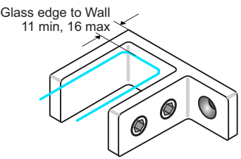
90 Deg Glass to Wall 65x55x25mm Part No JET/82/PSS Part No JET/82/SSS Part No JET/82/SCC
