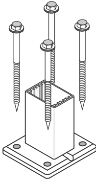
Top Mount Base Plates 110x90 or 110x110, 90deg Corner Post
