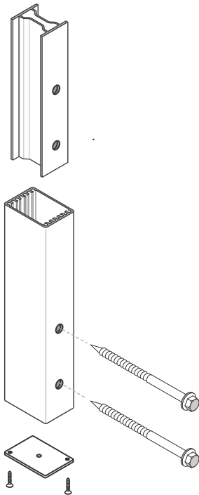
Face Fix Different fasteners types depending on the Building substrate.
