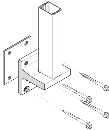
Gutter Bracket - Face Fixed Suitable for any overhanging decks and clearing Guttering channels.
