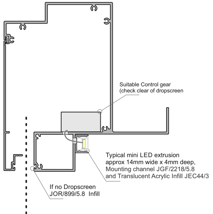
Perimeter Beam JOR/801 (With/without Dropscreen option)
