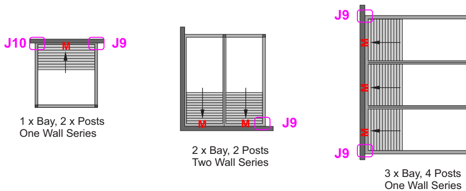
A Selection of some Layouts using Joint 9
