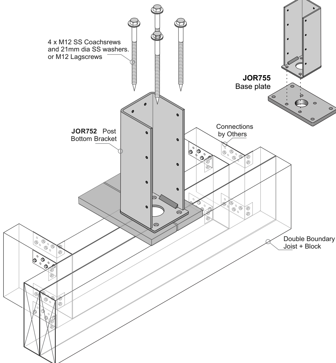
JOR752 Post Bottom Bracket + Optional Base Plates
