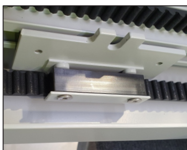
Belt pulled out of the way, to show Clamp
