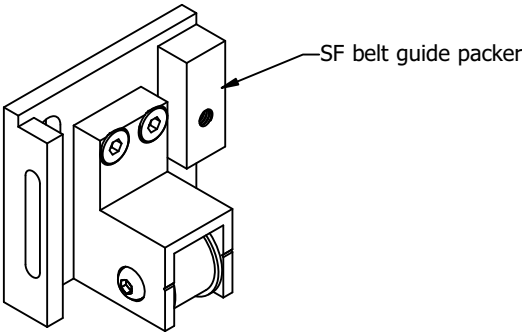
JOR957/LH SF Belt Guide Pelmet Assembly
