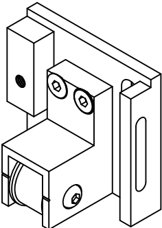
JOR957/RH SF Belt Guide Pelmet Assembly
