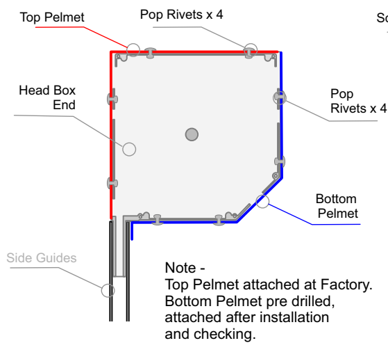
Pelmets, Headbox ends
