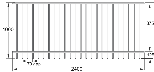
FENCE PANEL FP 10
