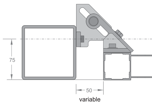
Bottom Hinge - Plan view
