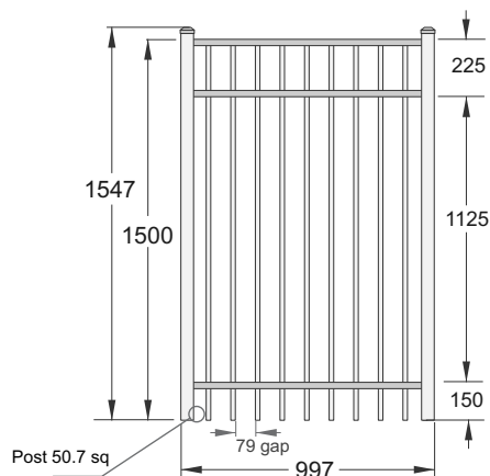
STANDARD GATE PANEL GP 15
