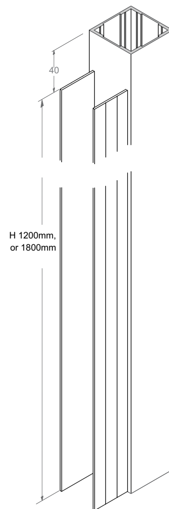
GATE END, Machined FPGE 1240, FPGE 1840
