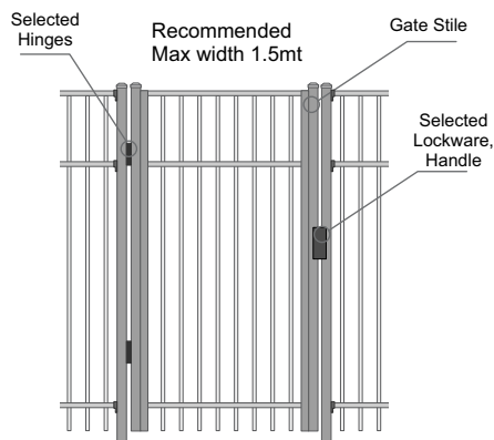
Typical Gate Plain
