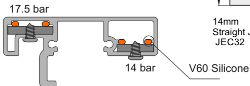
STANDARD HANDRAIL JEB/222/5.8
