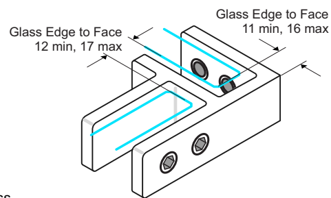
90 deg Glass to Glass 65x55x25mm Part No JET70/PSS Part No JET70/SSS Part No JET70
