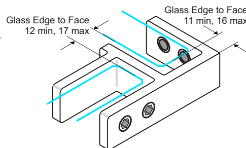
90 deg Glass to Glass 88x55x25mm Part No JET80/PSS Part No JET80/SSS Part No JET80
