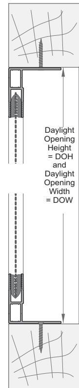
Reveal Fix
