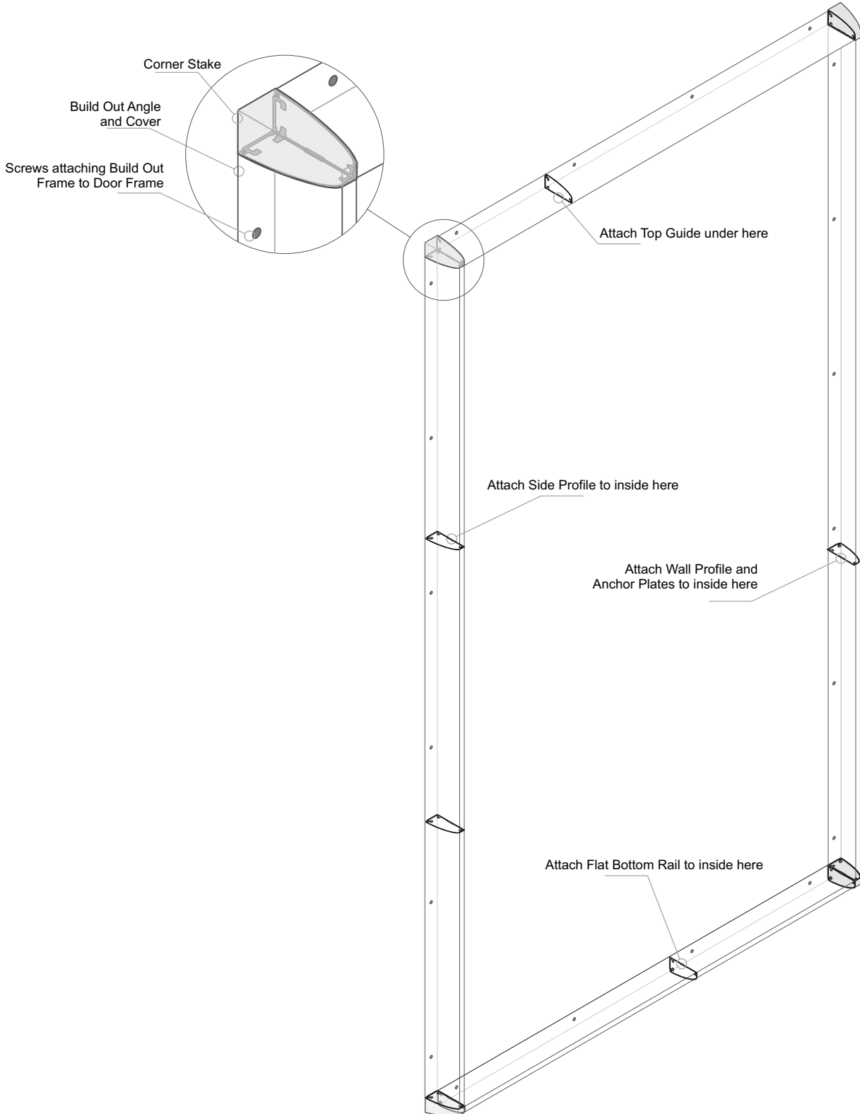
Build out angle Part No J7468
