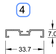
MAGNET HOLDER 4.9m JMX/08-00070-0-0
