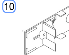
Guide plate for Sliding Bar Top Cap JMX/08-13330-0-5
