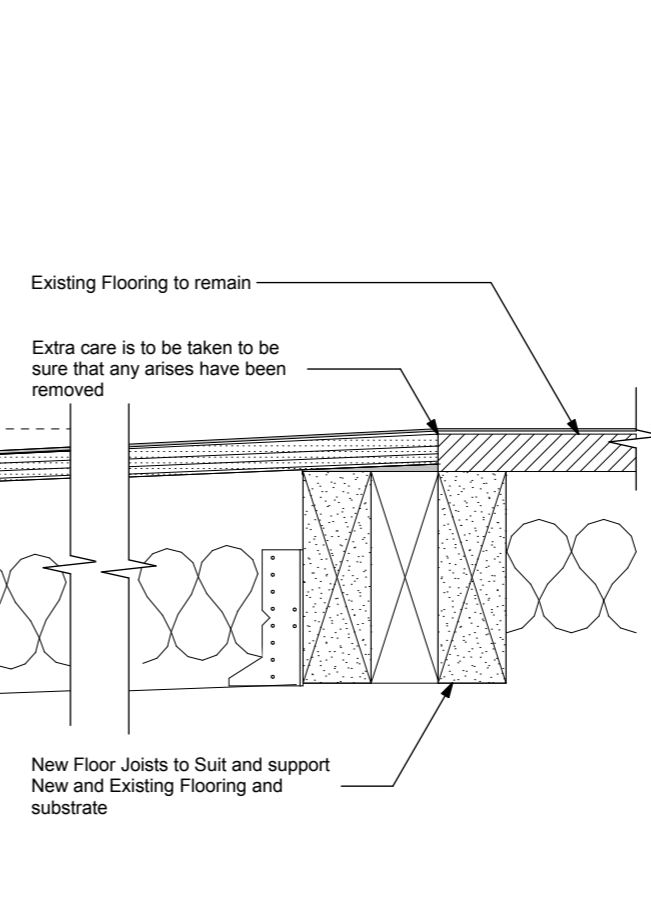
Bathroom (Non wet area) Floor to Wall Detail
