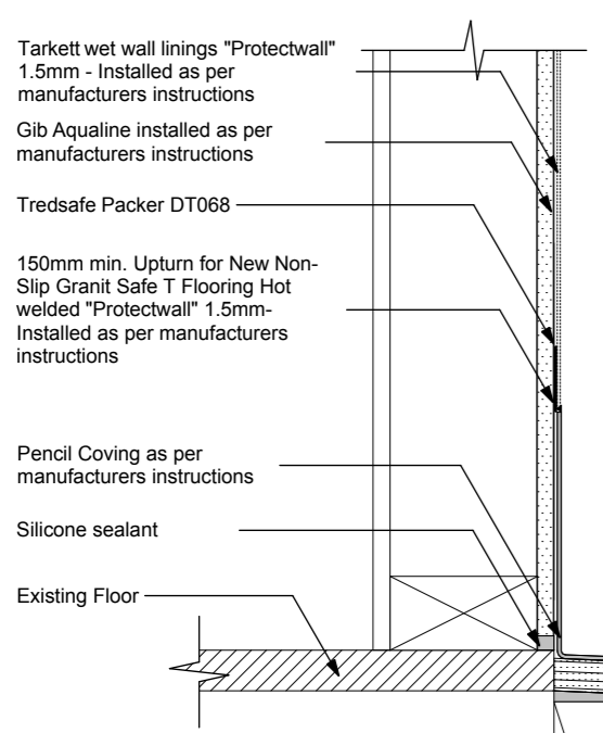
W.A.S Shower Floor to Wall Detail
