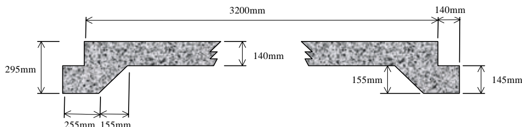
Figure 4: Concrete slab
