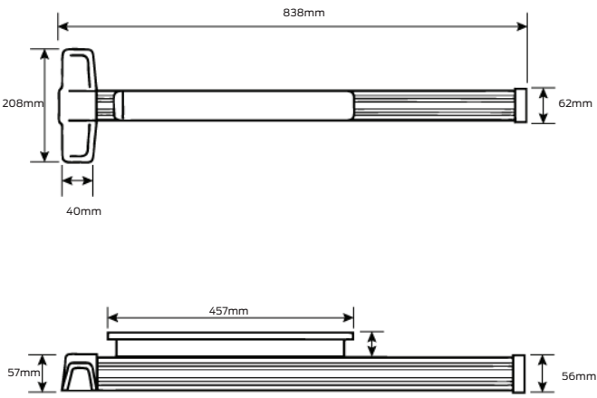
Device centre line to finished floor: 1011mm
