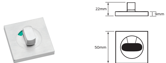
Indicating turn #8013
