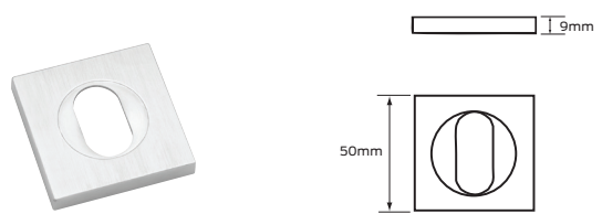
Cylinder #8008
