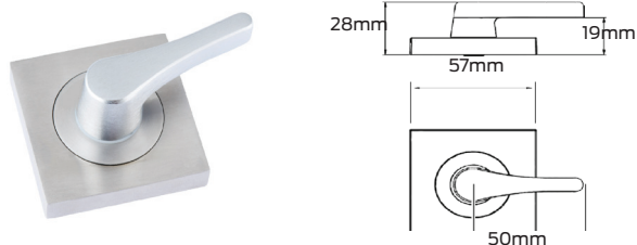
Accessible turn #8054
