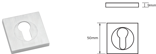
Euro profile cylinder #8012
