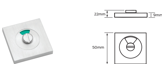
Indicating emergency release #8014
