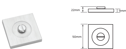
Emergency release #8009
