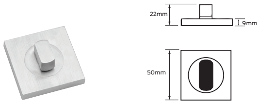
Emergency release #8009
