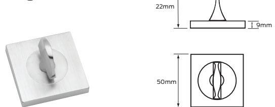
Large turn #8010
