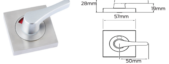
Indicating accessible turn #8054IND
