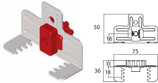
MBFR Adjustable Direct Fix Furring Channel Resilient Mount
