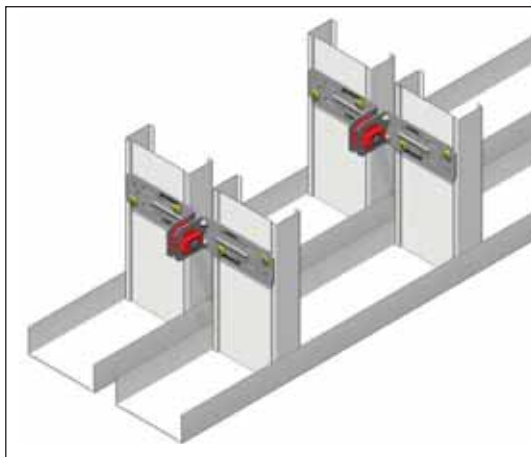
M24R Resilient mount shown installed in a chase wall to improve the strength and rigidity of the chase walls, allowing both walls to support each other whilst remaining completely isolated.
