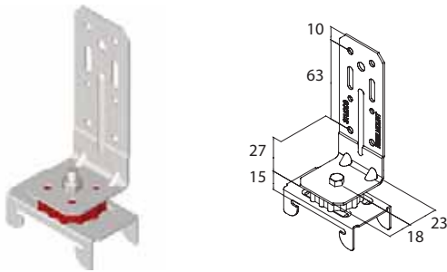
M96R Furring Channel to Purlin Resilient Mount
