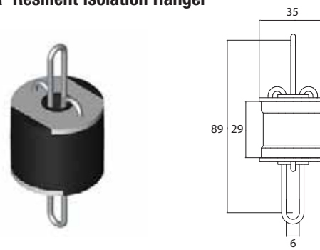
M50R Resilient Isolation Hanger
