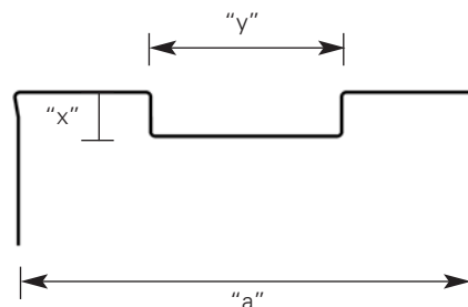
Fig. 3 Custom Cavkit Closer Cap - Specify the 'x', 'y' and 'a' dimensions to suit project requirements
