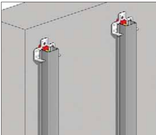
MBFR Adjustable resilient mount shown direct fixed to concrete walls. MBFR clips have adjustment of 4 positions at 6mm increments to adjust furring channels, eliminating packers.
