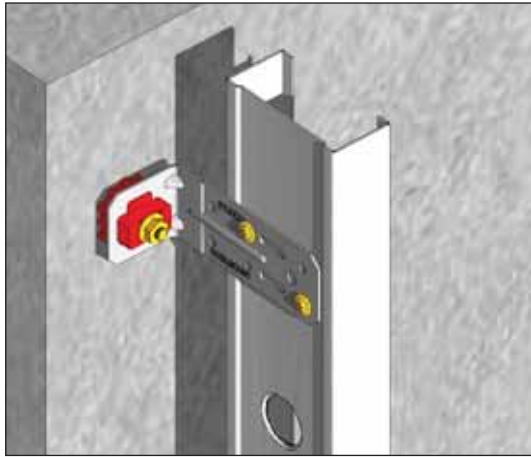
M48R Resilient mount shown direct fixed to the structure, to brace an acoustic wall to the structure without compromising sound and vibration transmission requirements.
