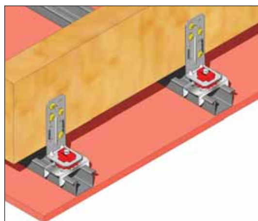
M96R Resilient mount shown fixed to purlins or trusses, for the suspension of furring channels. 5mm slotted holes are provided in bracket for adjustability.
