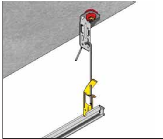
M48R Resilient mount shown with 5mm suspension rod attached for isolation of ceiling from structure.
