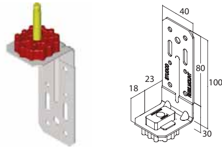
M48R Resilient Mount Right Angle Bracket
