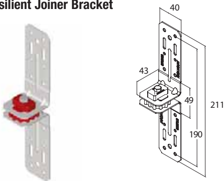
M24R Resilient Joiner Bracket
