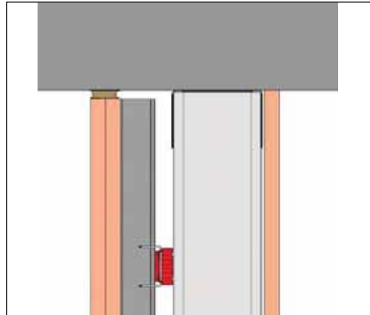
M237R Resilient clip shown direct fixed to steel stud to provide greater acoustic ratings.
