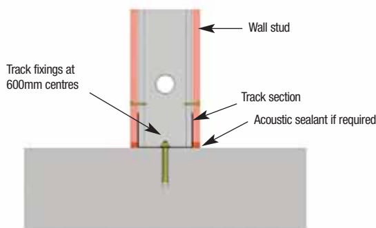
Fig. 1 Bottom Track Fixing
