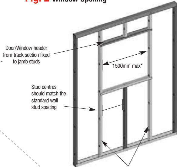
Fig. 2 Window Opening
