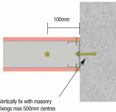
Fig. 3 Wall End Intersection to Concrete
