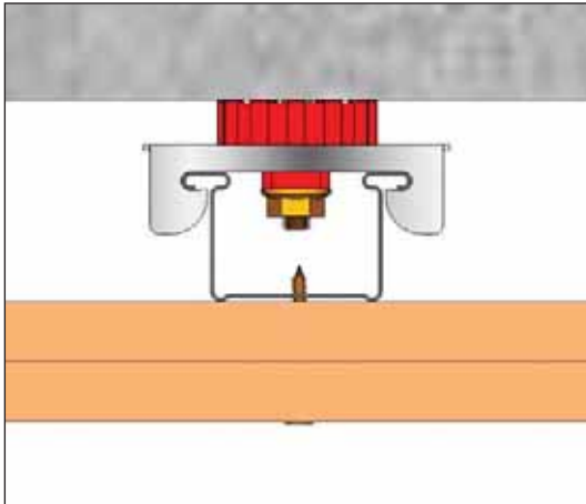
M237R Resilient mount shown direct fixed to concrete to provide isolation for wall & ceiling applications
