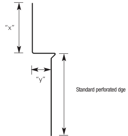
Fig. 2 Custom Shadowline - specify the 'x' and 'y' dimension to suit project requirements
