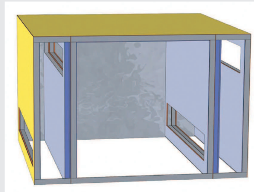
Typical enclosure construction showing air inlet/outlet
