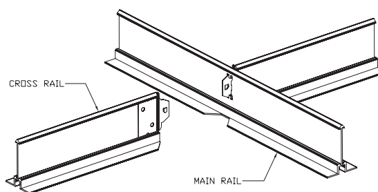
Armstrong “Blue Tongue” positive lock connection.
