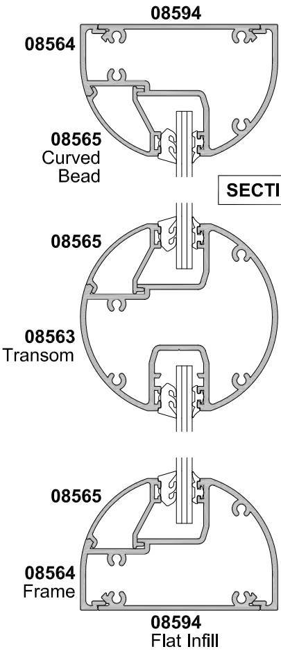
SECTION B-B
