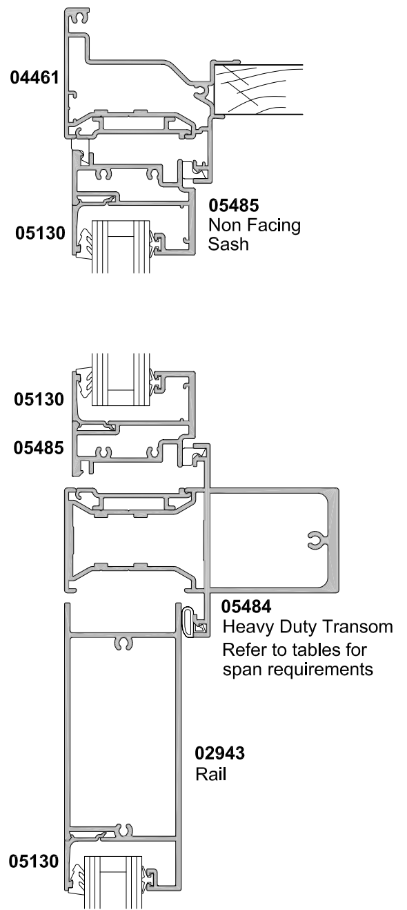
SECTION B-B
