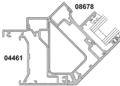
04443 135° COUPLING BAR
