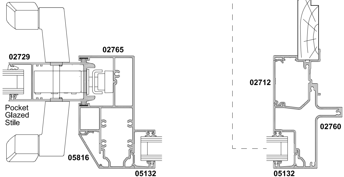
MORTICE LOCK OPTION
