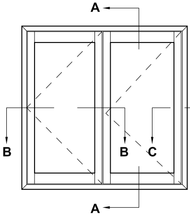
STANDARD BI-FOLD
