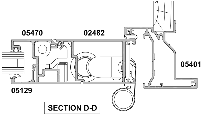
STANDARD BI-FOLD
