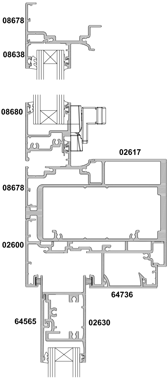
SECTION A-A COUPLED METRO AWNING FRAME
