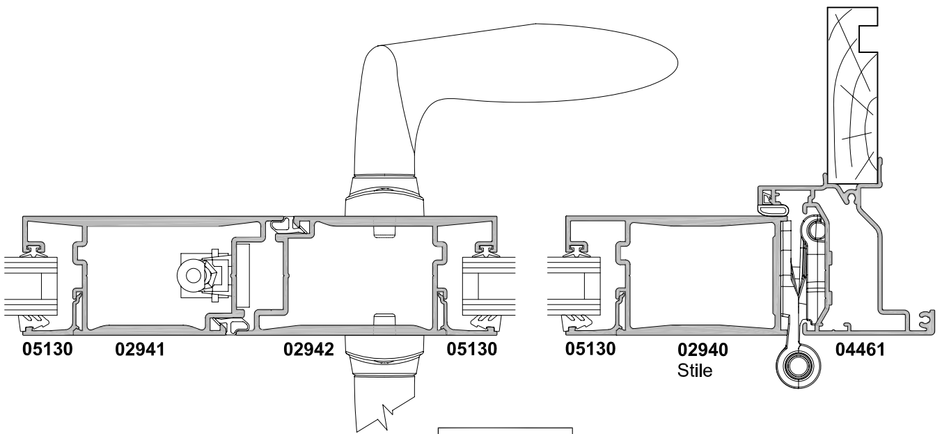
SECTION A-A OPEN OUT FRENCH DOOR
