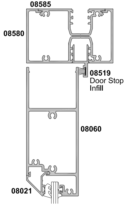
SECTION C-C
