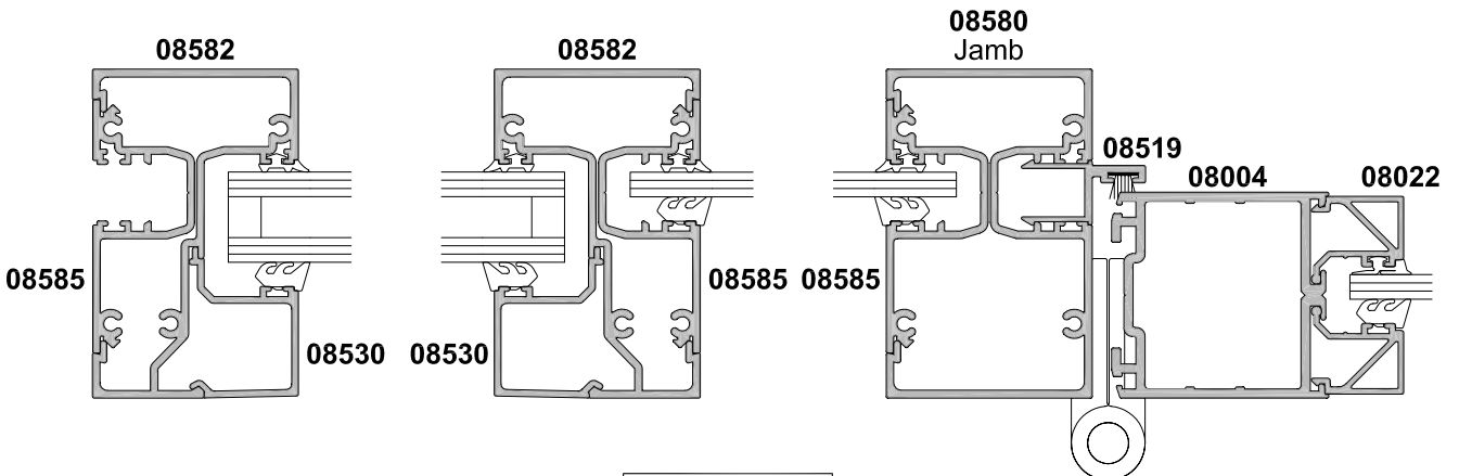
SECTION B-B
