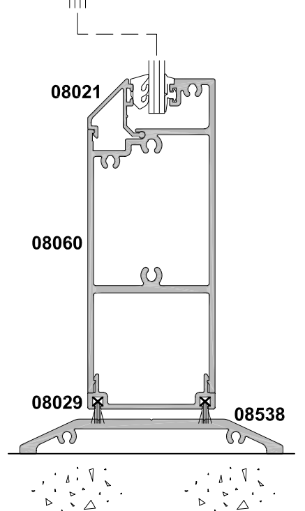
SECTION F-F
