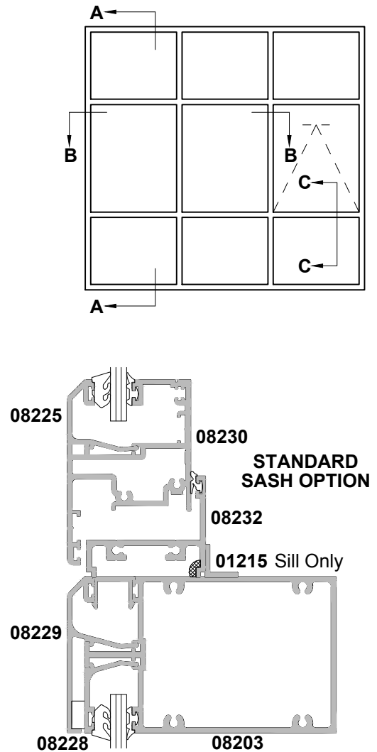
SECTION C-C
