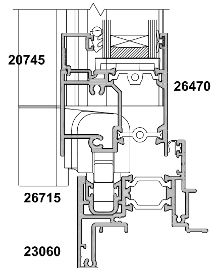
SMALL FLUSH RAIL OPTION (WINDOW RAIL)
