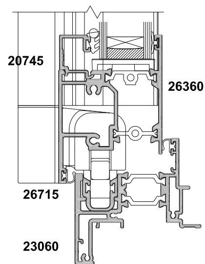
SMALL RAIL OPTION (WINDOW RAIL)
