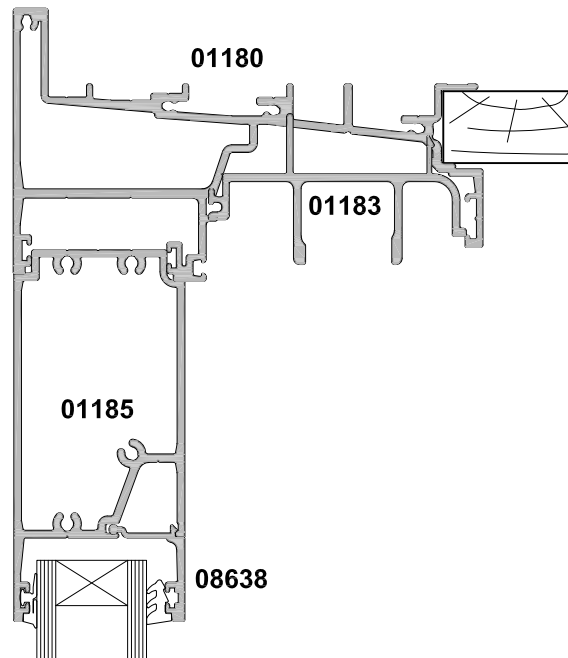
SECTION B-B
