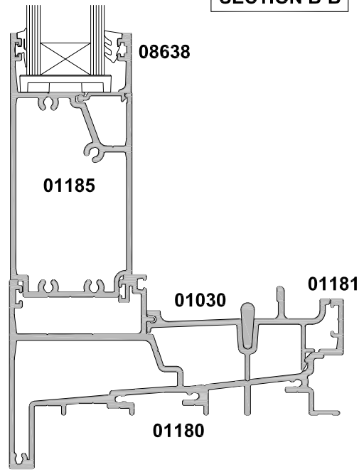
SECTION B-B
