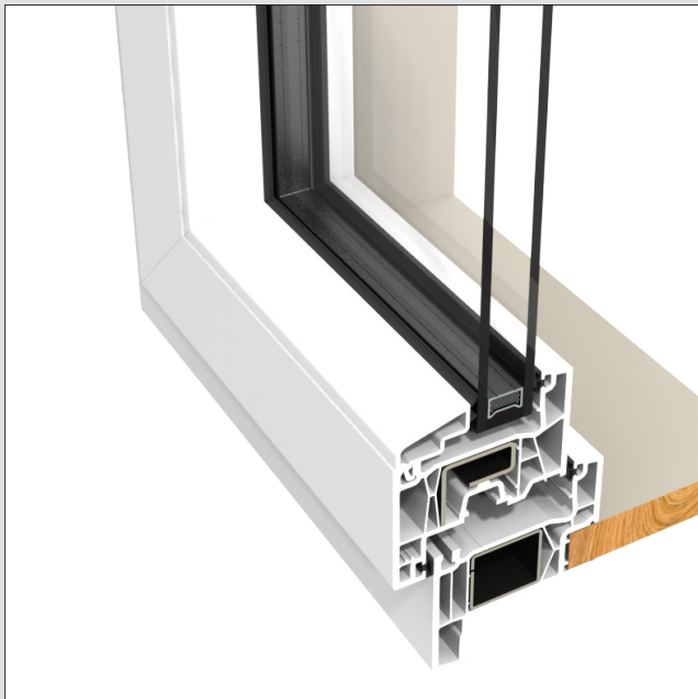
Standard window frame with awning sash.
