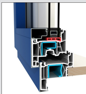
Window frame and sash with Aluclip exterior.
