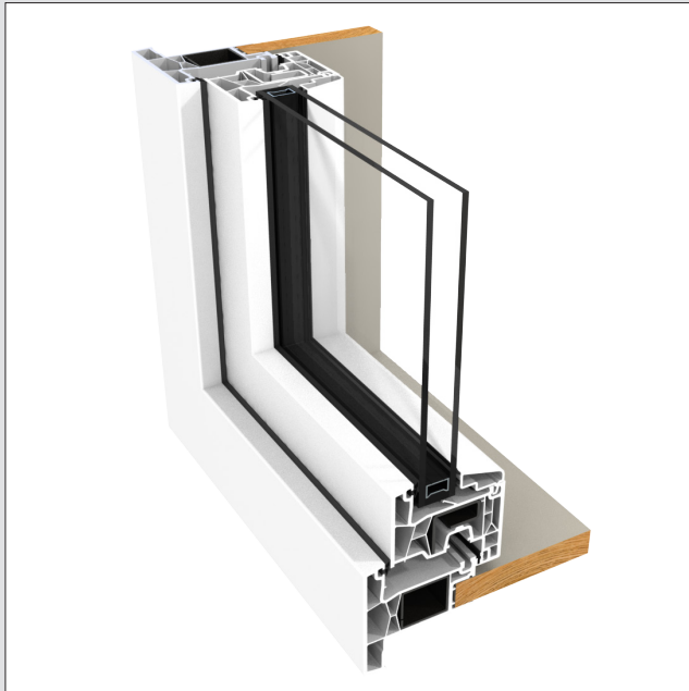
Tilt and turn frame and sash.
