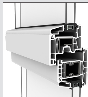
Awning sash and transom - exterior view.
