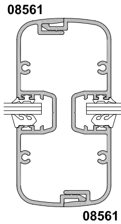
SECTION B-B
