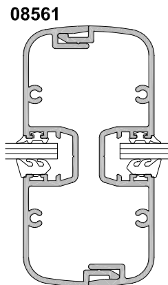
08561 Split Mullion
