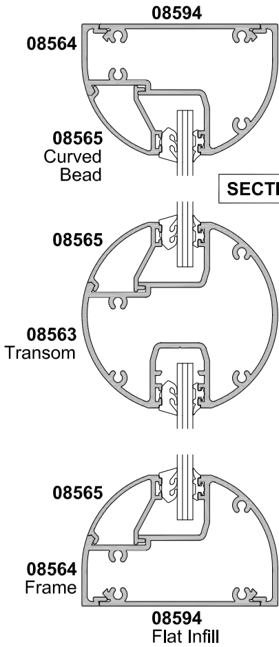
SECTION B-B
