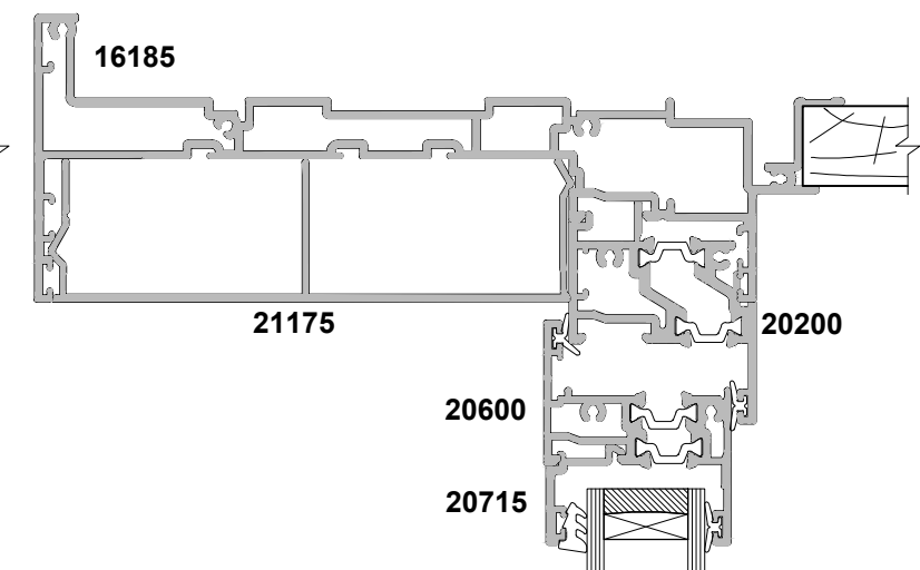
SECTION C-C
