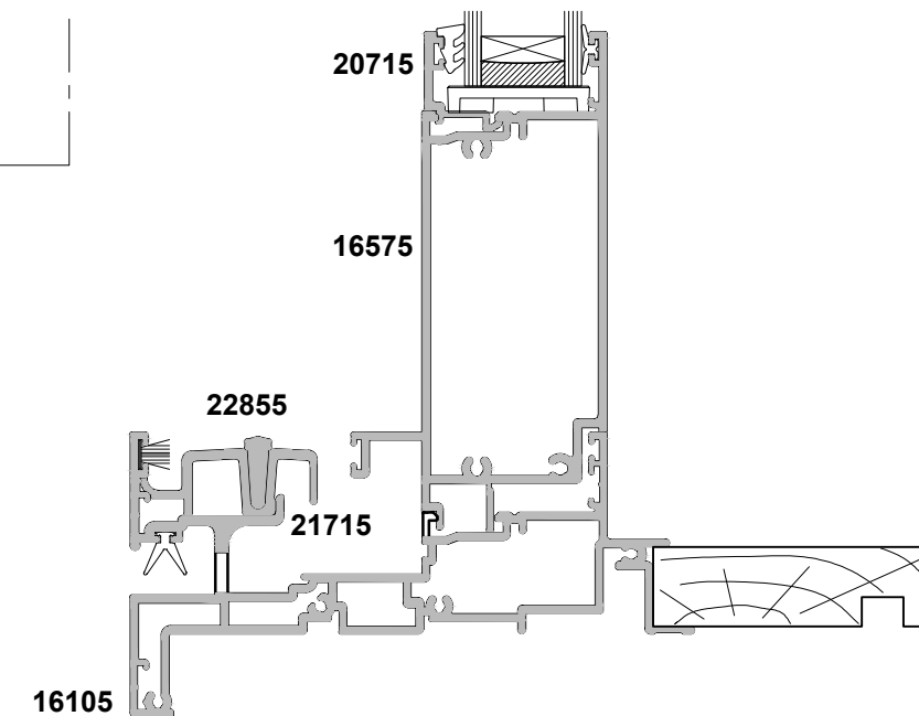
VISION RAIL OPTION
