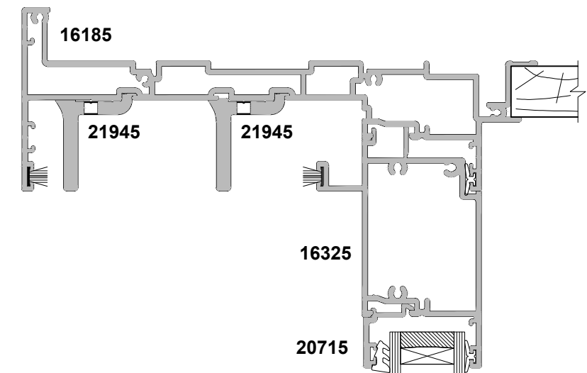
SECTION C-C
