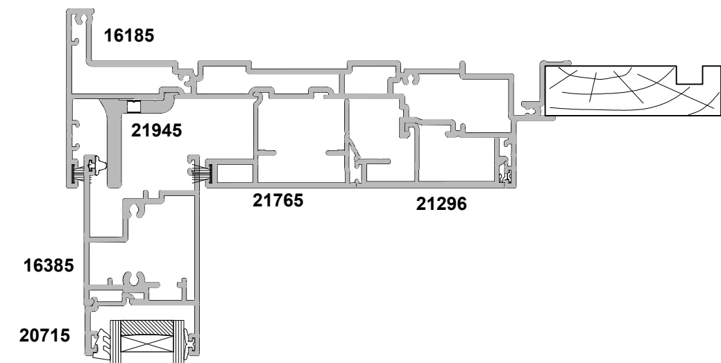
SECTION B-B
