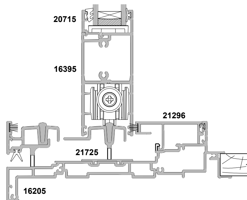
SECTION B-B
