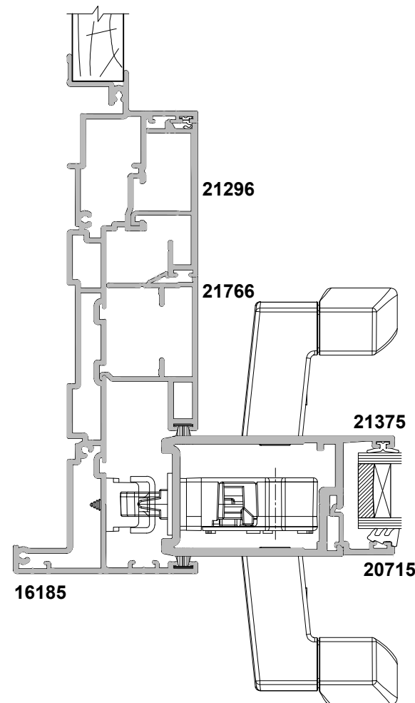
STANDARD D-PULL OPTION
