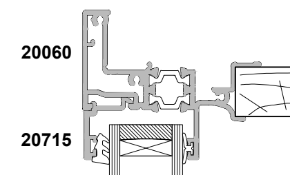
SECTION B-B COUPLER OPTION
