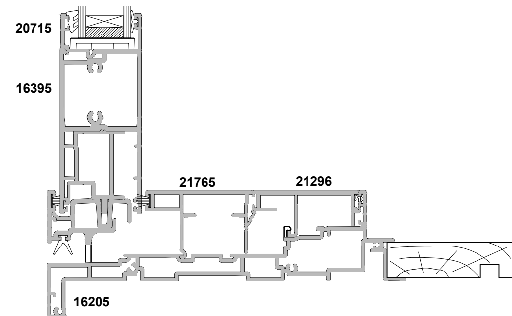
SECTION B-B
