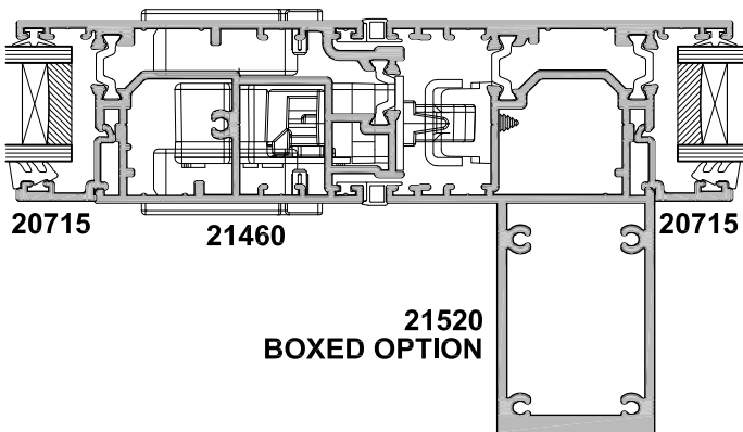
FLUSHPULL HANDLE OPTION
