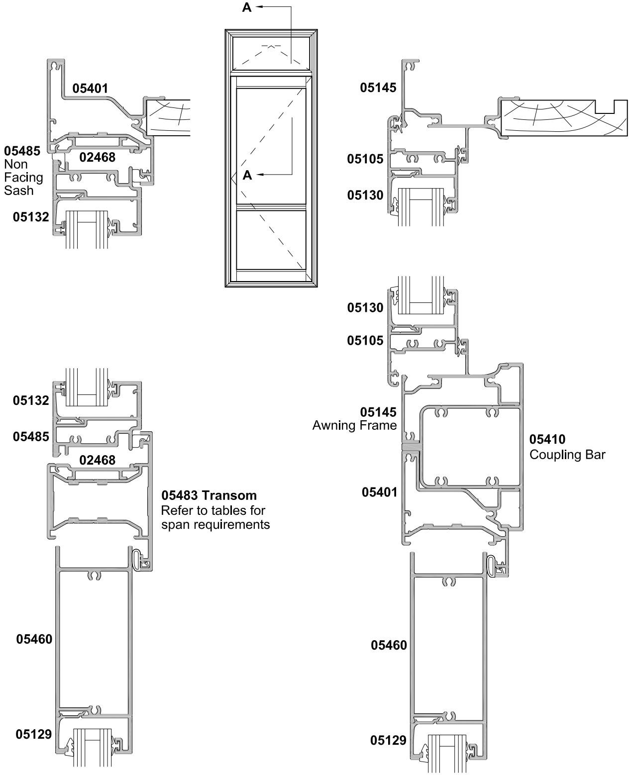
SECTION A-A OVERLIGHT TRANSOM OPTION
