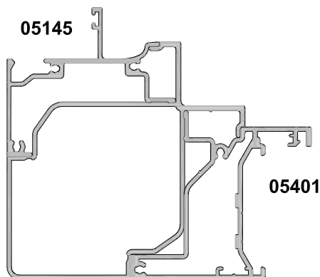
05412 90° Corner Coupling
