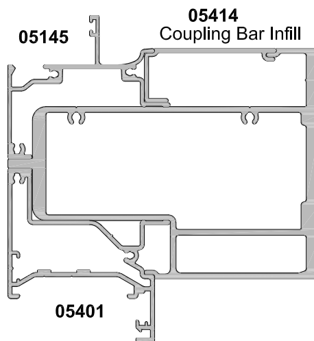
05413 Heavy Duty Overlight Coupling Bar
