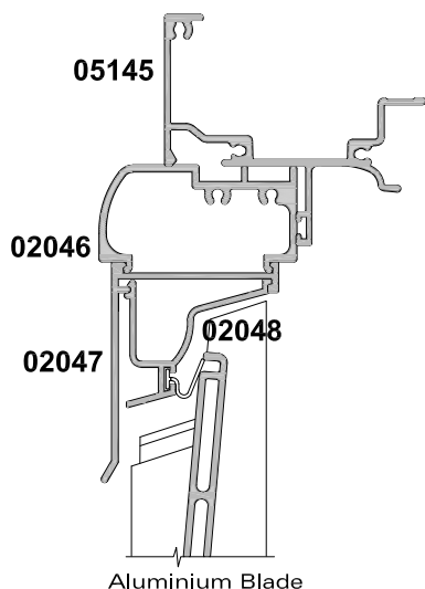
Aluminium Blade
