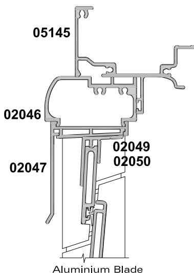
Aluminium Blade
