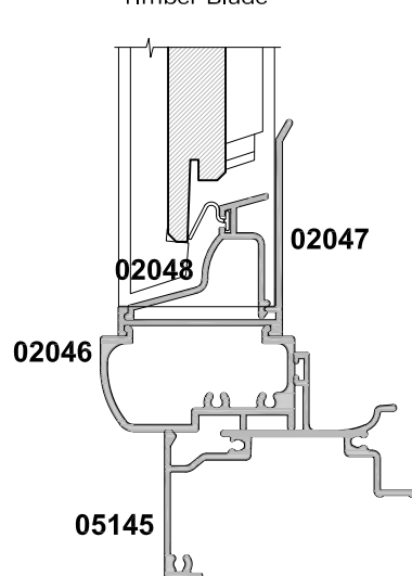
Timber Blade
