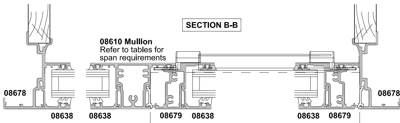
VENTED SASH OPTION
