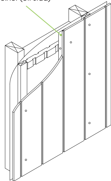
Weathergroove joiner (off stud)
