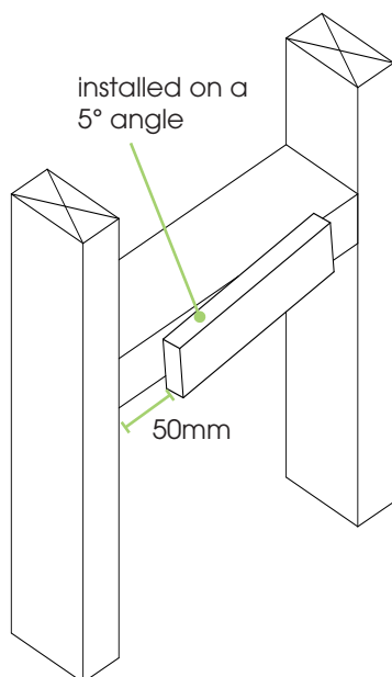
CAVITY SPACER
