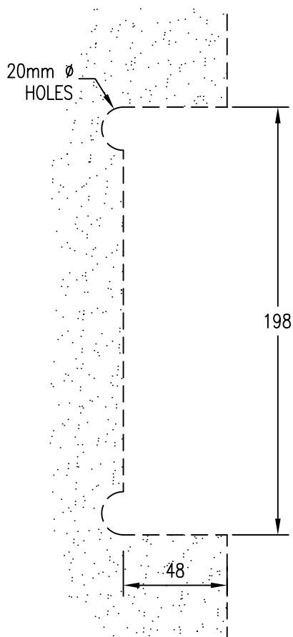
GLASS PREPARATION
