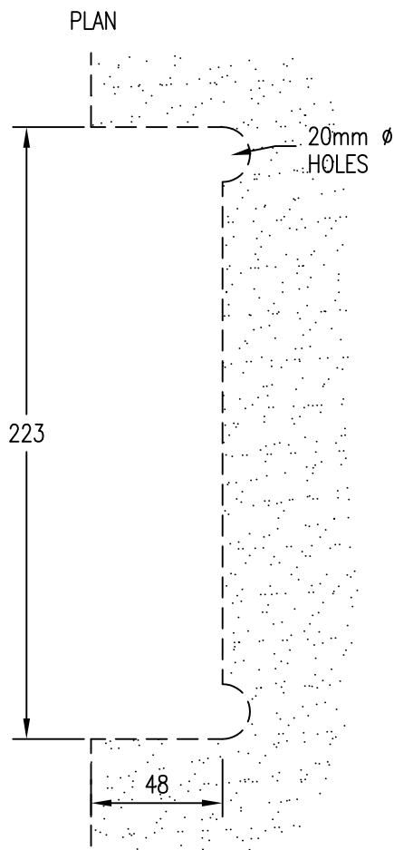
GLASS PREPARATION
