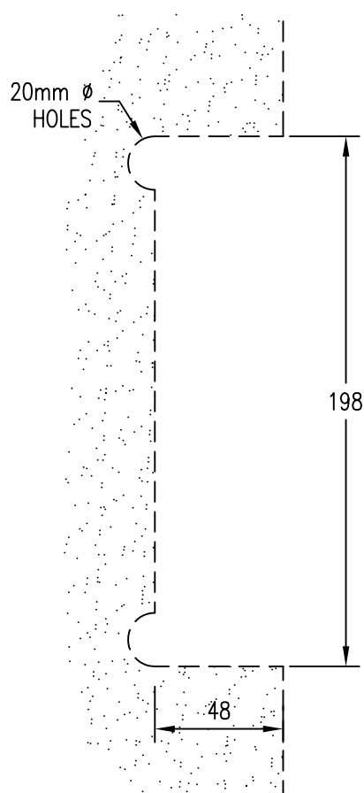
GLASS PREPARATION
