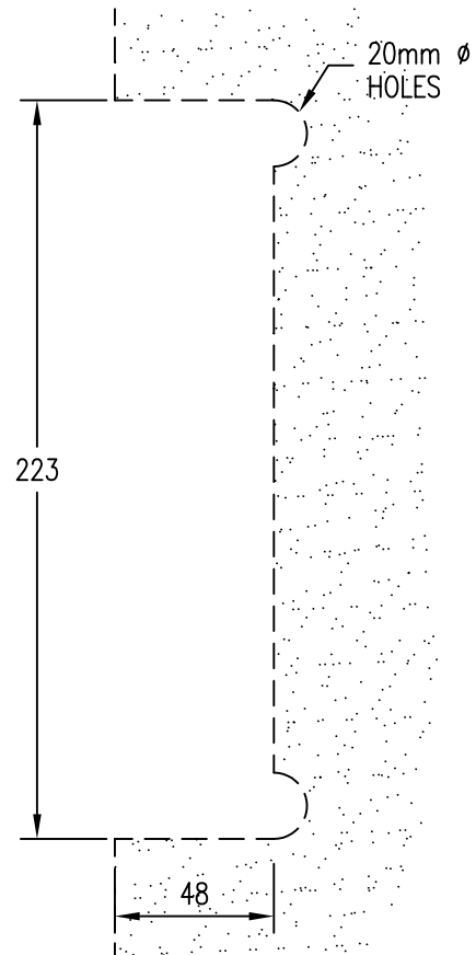
GLASS PREPARATION
