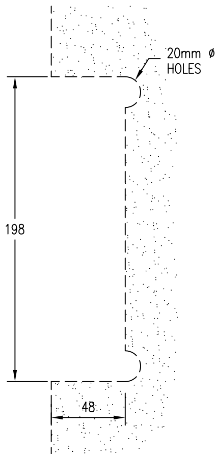
GLASS PREPARATION
