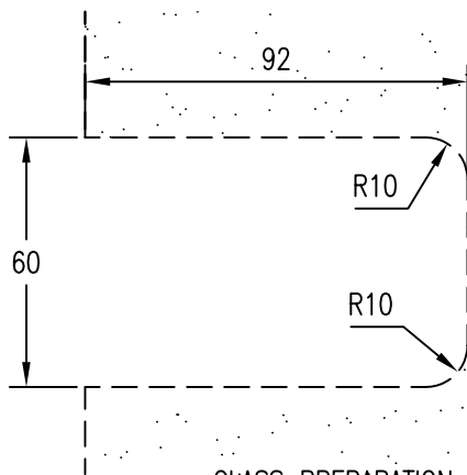
GLASS PREPARATION
