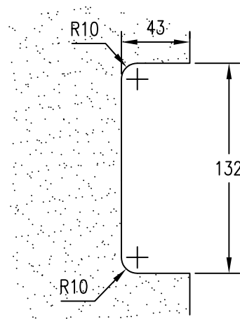
GLASS PREPARATION US20 & GK50
