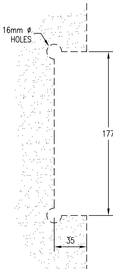
GLASS PREPARATION
