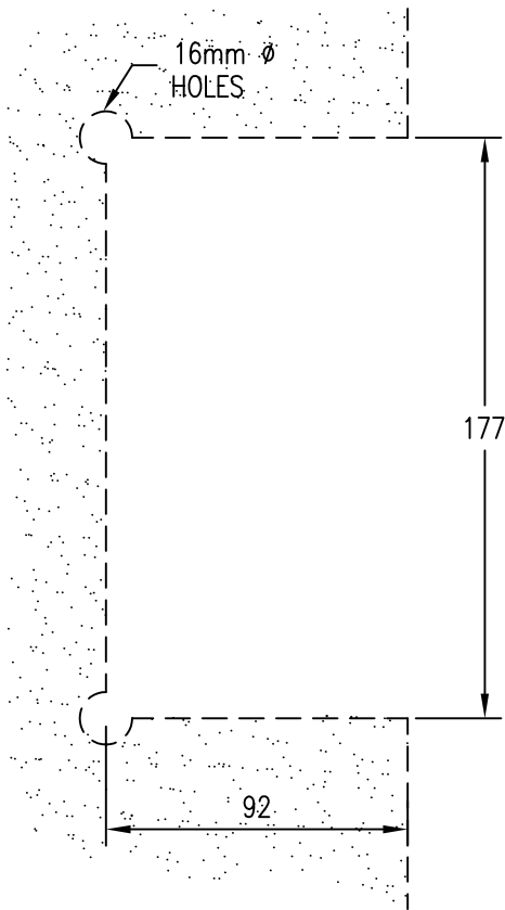
GLASS PREPARATION
