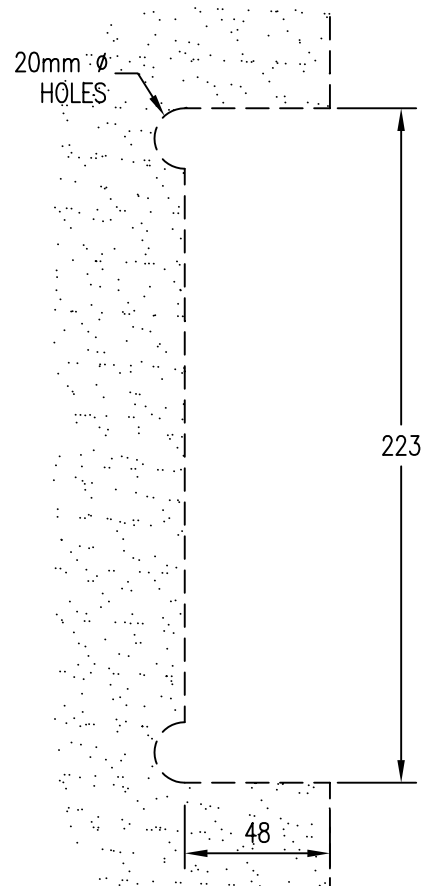
GLASS PREPARATION
