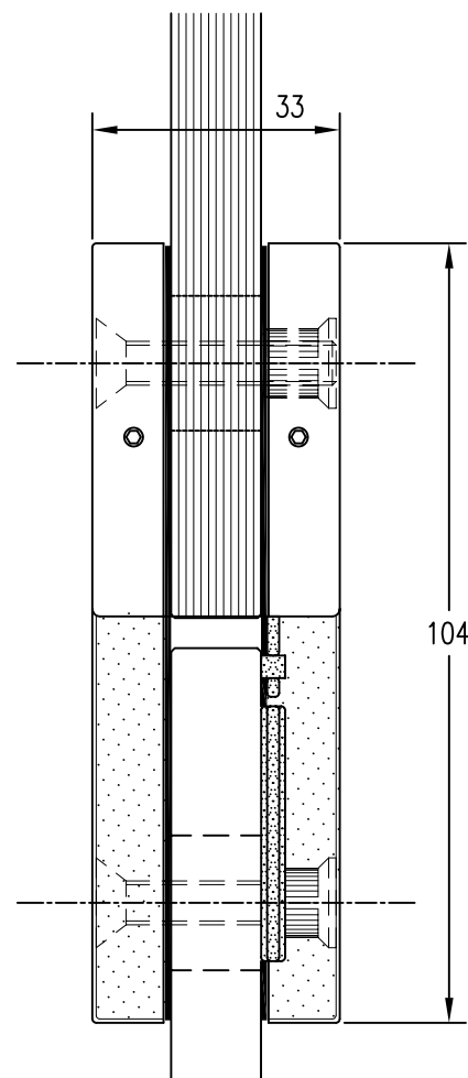
END VIEW
