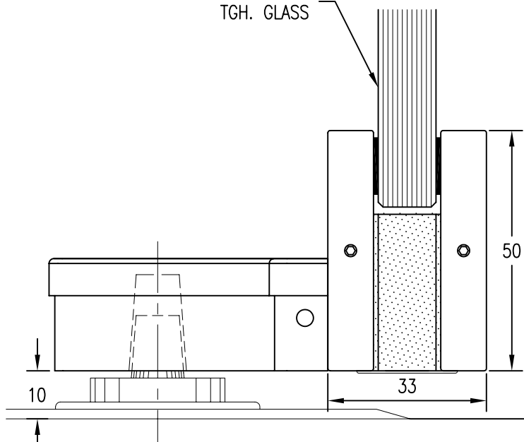
END VIEW
