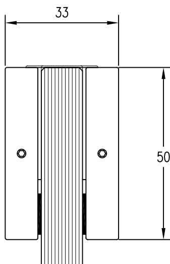
END VIEW
