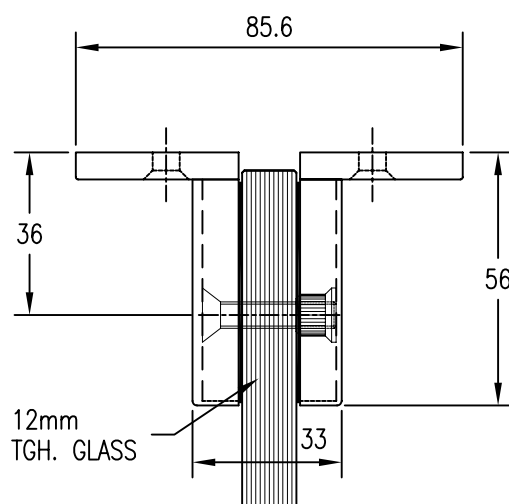
SECTION
