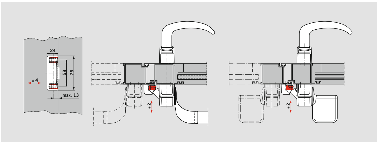
Application example of a PHX 21 on a door with flush meeting stiles, universal applicability for single-leaf and double-leaf doors
