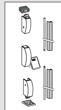
2-point locking
