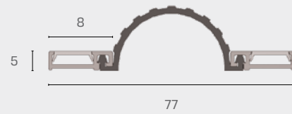
IS9055 Finger Guard Seal - hinge position
