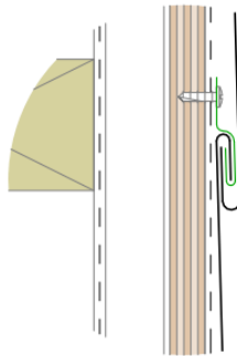
Euro Wall Hook Seam Horizontal
