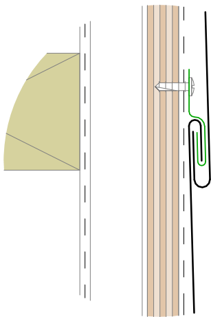
Euro Wall Hook Seam Horizontal
