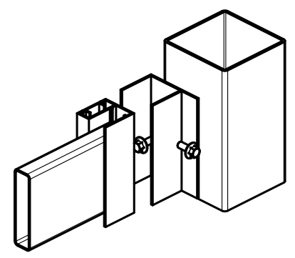
FRESNO PANEL TO POST DETAIL 1:4
