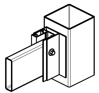
FRESNO PANEL TO POST DETAIL 1:4
