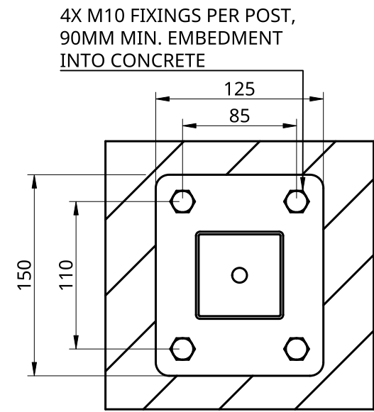
BASEPLATED POST CONNECTION
