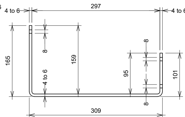
285 - 300 BOX GUTTER BRACKET
