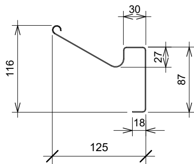
125 BOX GUTTER INTERNAL BRACKET
