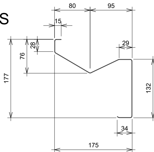
175 BOX GUTTER INTERNAL BRACKET
