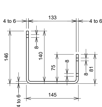
125 BOX GUTTER BRACKET
