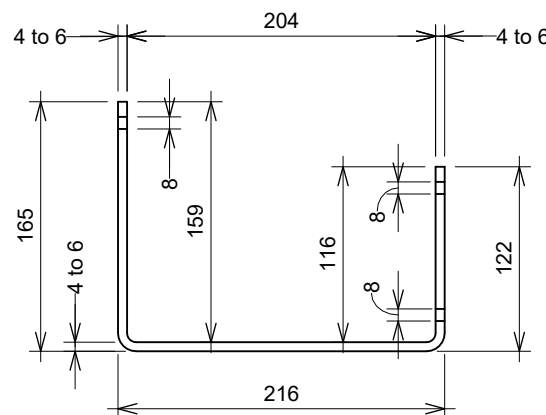
175 BOX GUTTER BRACKET
