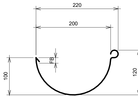
ROOFING INDUSTRIES 200mm HALF ROUND GUTTER
