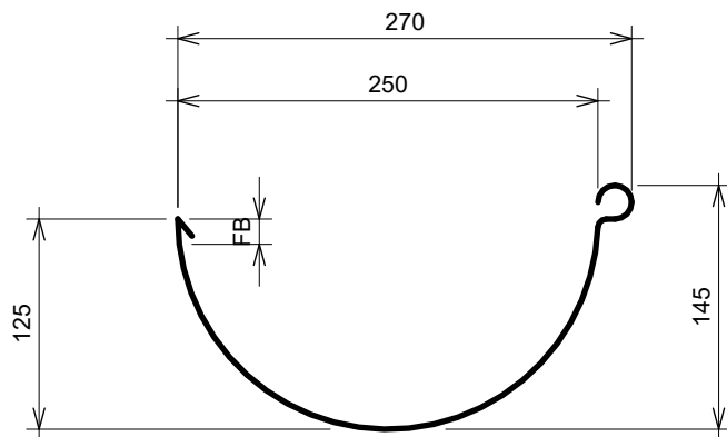
ROOFING INDUSTRIES 250mm HALF ROUND GUTTER
