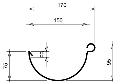
ROOFING INDUSTRIES 150mm HALF ROUND GUTTER
