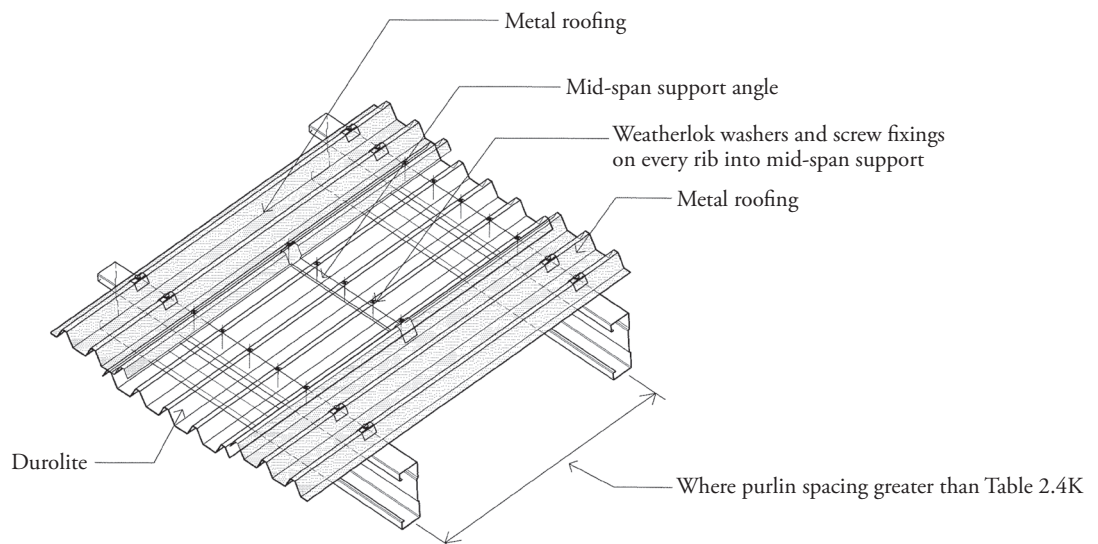
FIG 12 MID-SPAN SUPPORT DETAIL (ALL PROFILES EXCEPT DECKING)
