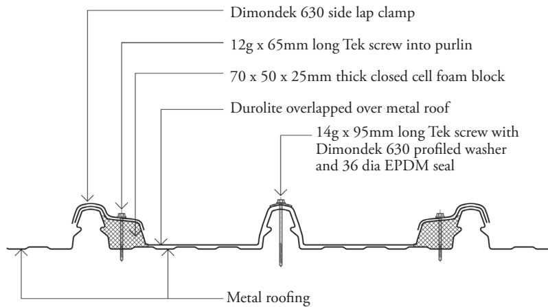
FIG 10 DUROLITE DIMONDEK 630 ENDLAP OVER METAL ROOFING
