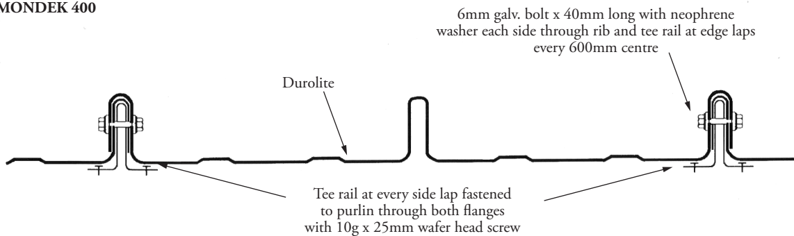
FIG 9 MULTIPLE DUROLITE SHEET DETAIL WITH DIMONDEK 300 OR DIMONDEK 400
