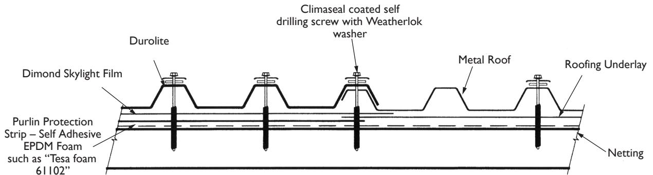
FIG 1 DIMOND SKYLIGHT FILM DETAIL
