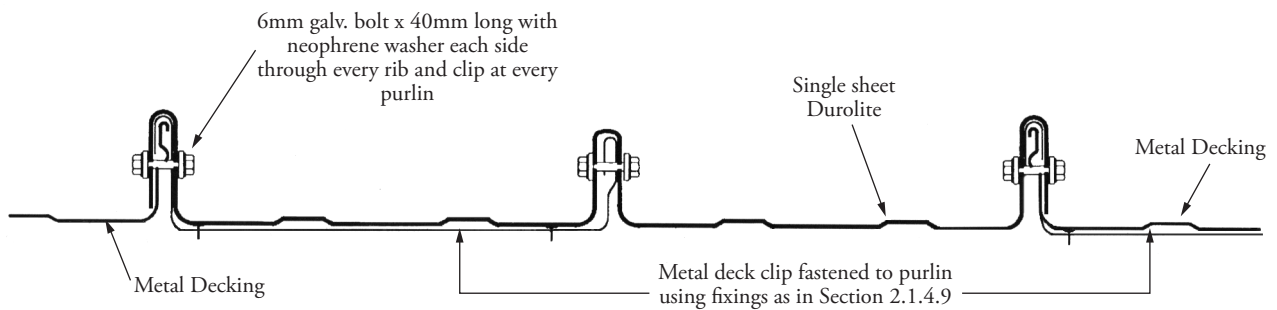
FIG 8 DETAIL FOR SINGLE DUROLITE SHEET WITH DIMONDEK 300 OR DIMONDEK 400
