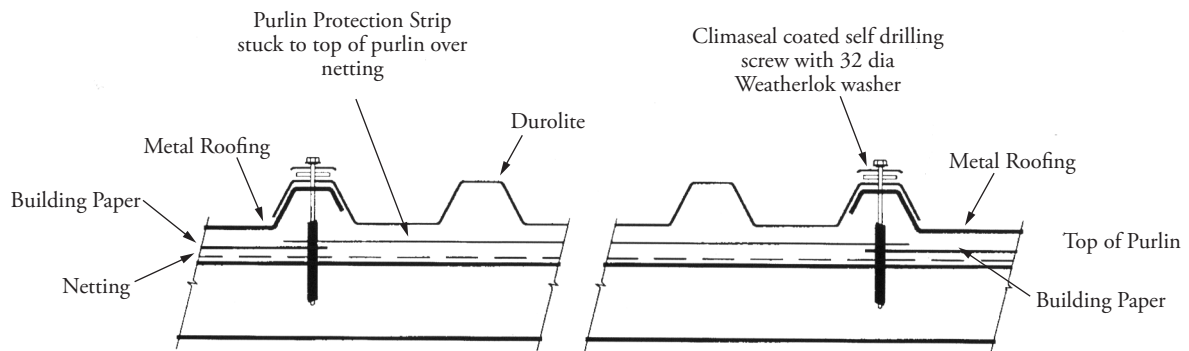
FIG 6 SIDE LAP DETAIL OF DUROLITE WITH METAL ROOFING (OVER/OVER PROCESS)
