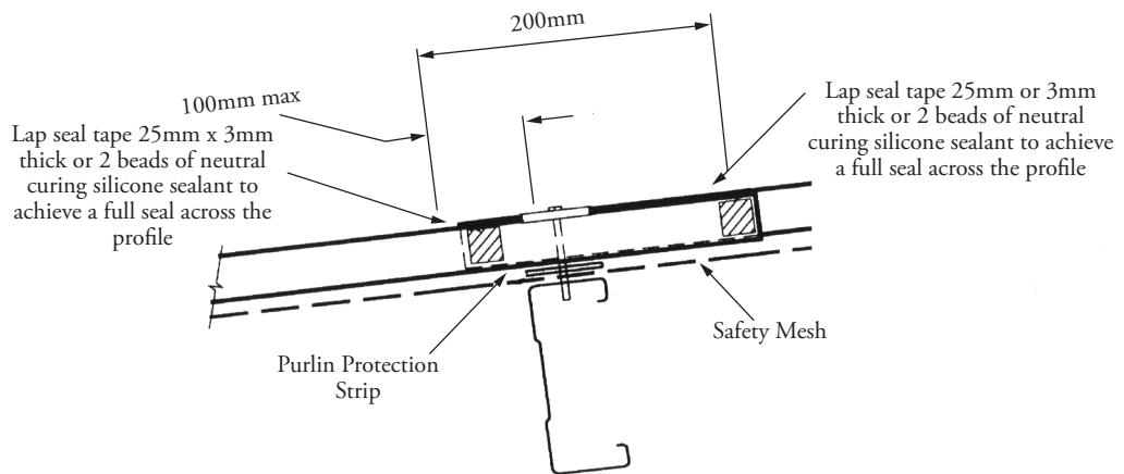
FIG 4 END LAP DUROLITE TO DUROLITE & DUROLITE TO STEEL
