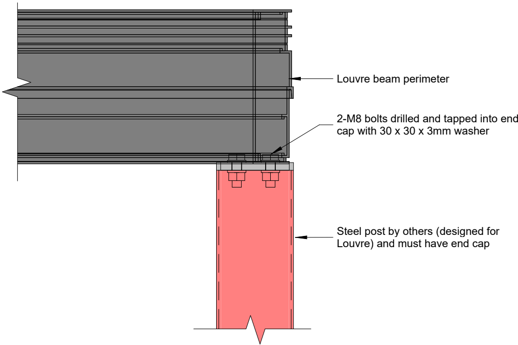
LOUVRE TO POST DETAIL 1 : 5
