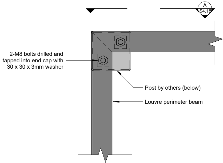
LOUVRE TO POST DETAIL 1 : 5
