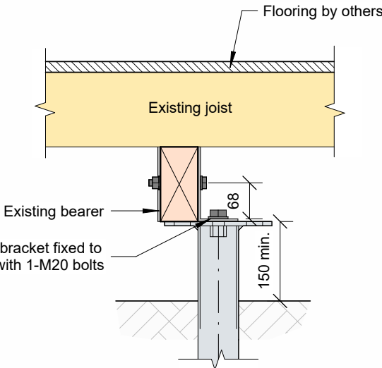
B PILE CONNECTION S4.16 1 : 10
