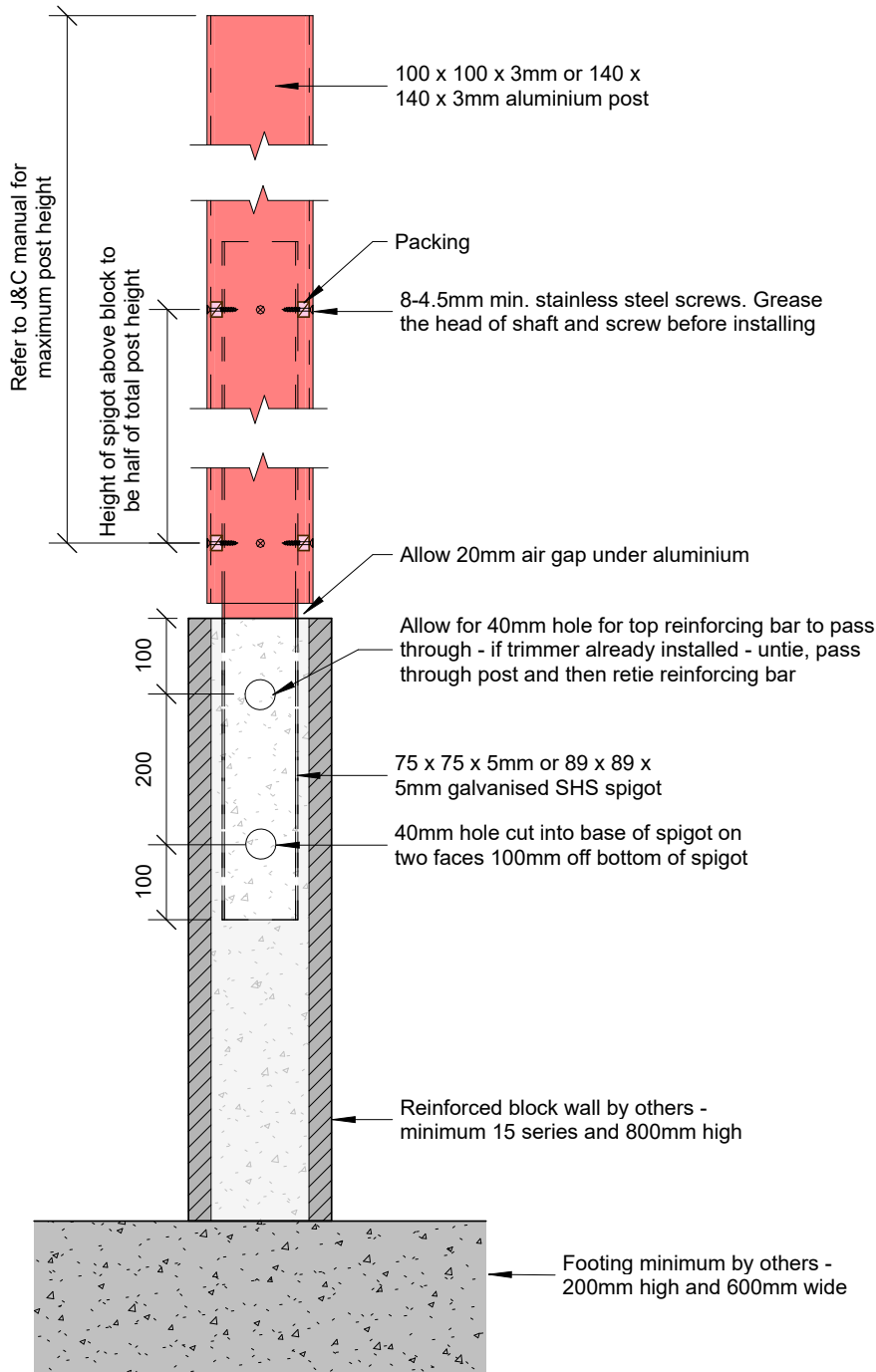
BLOCK ON SLAB 1 : 10
