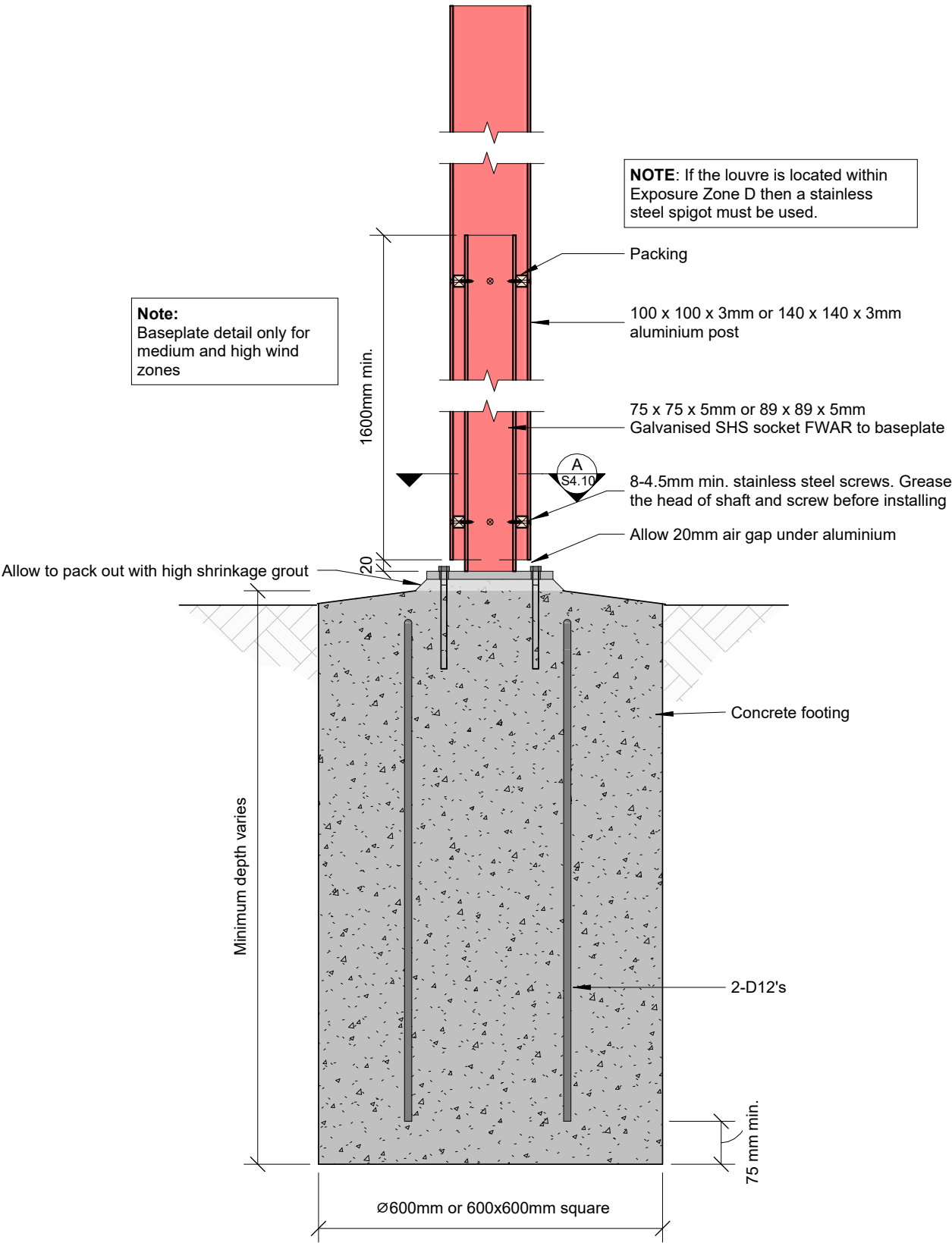
BRACED CANTILEVER POST FOOTING 1 : 10
