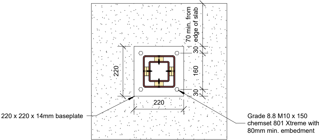
A CANTILEVER FOOTING S4.10 1 : 10
